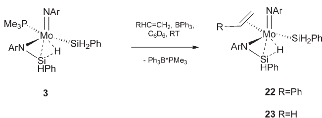
Scheme 12. Reactions of 3 with Olefins in the Presence of \text{BPh}_3
