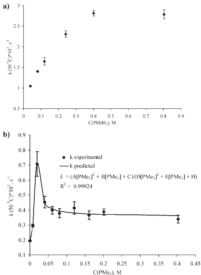
Figure 6. Dependence of the rate constant of the reaction of 17 with \text{PhSiH}_3 (10 equiv of \text{PhSiH}_3 ) at 50\text{ }^\circ\text{C} on (a) the concentration of \text{PhSiH}_3 and (b) the concentration of \text{PMe}_3 .
