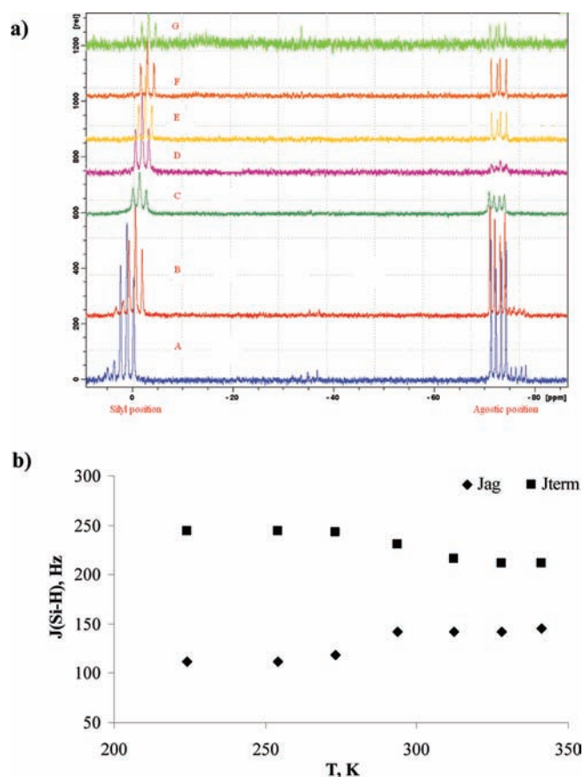
Figure 1. (a) ^{29}\text{Si} INEPT+ NMR spectra of 3 at -49 (A), -19 (B), 0 (C), 21 (D), 39 (E), 55 (F), and 68 °C (G). (b) Effect of temperature on the ^1J_{\text{Si-H}} values for the agostic silyl center in 3 .
