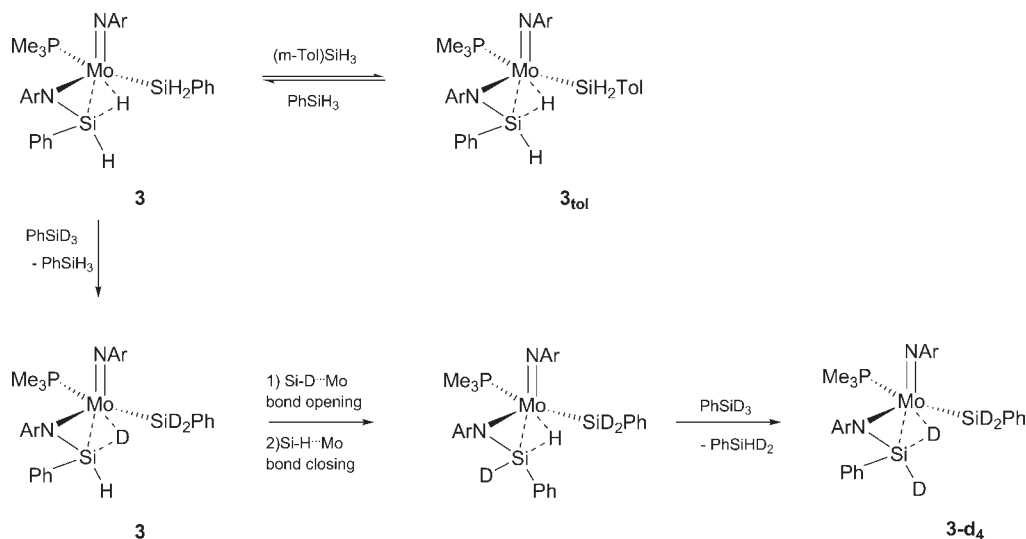
Scheme 4. Exchange of 3 with ( m -Tol)SiH 3 and PhSiD 3
