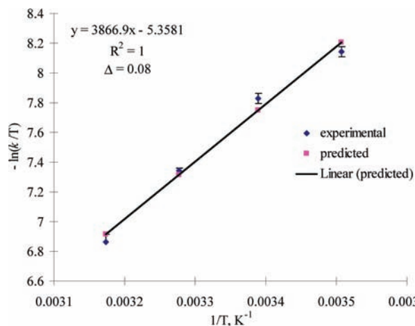
Figure 3. Eyring plot for the exchange between 3 and PhSiH 3 (standard error: 0.08).
