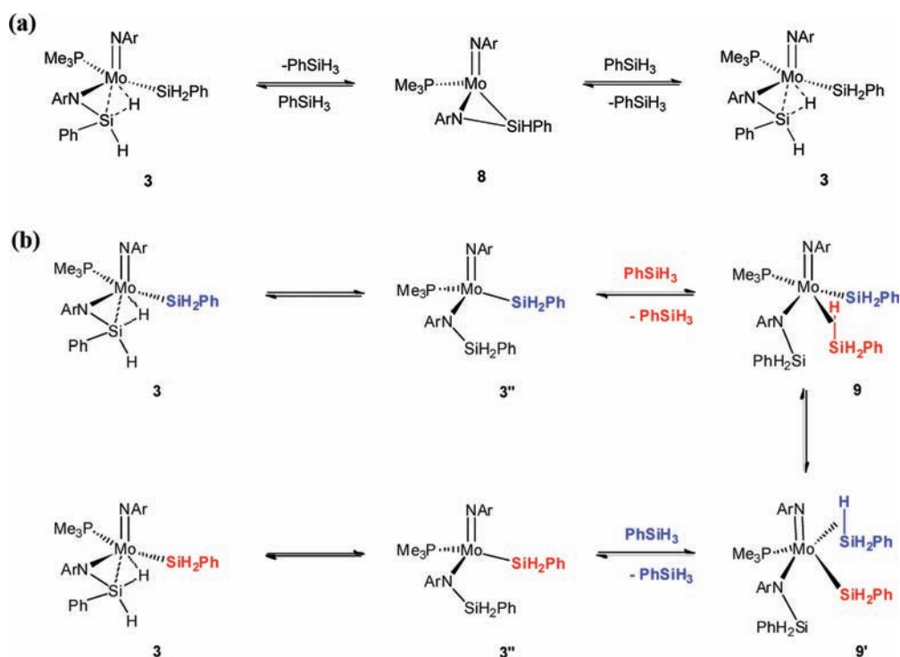
Scheme 5. Silane/Silyl Exchange in 3 via (a) Silanimine Intermediate 8 (Dissociative Mechanism) and (b) an Associative Mechanism
