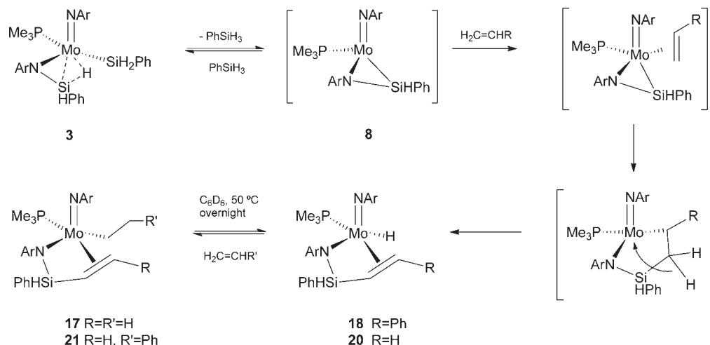
Scheme 11. Suggested Mechanism of the Reaction of Complex 3 with Olefins
