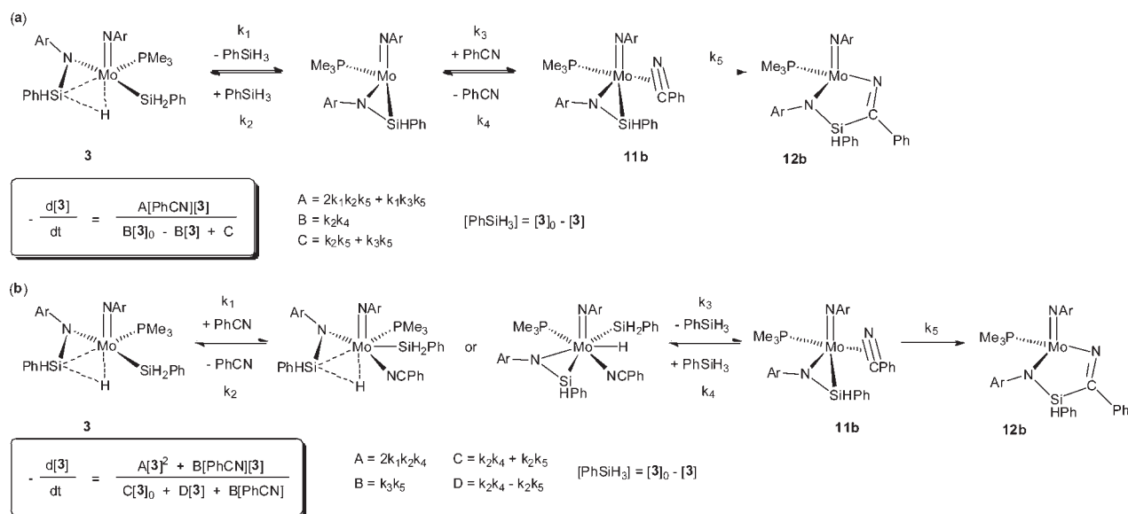
Scheme 7. Possible Mechanisms, Dissociative (a) and Associative (b), for the Reaction of 3 with PhCN
