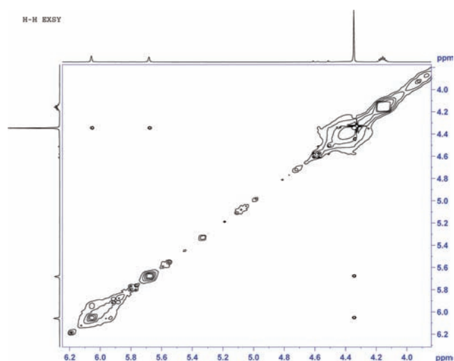
Figure 2. ^1\text{H} – ^1\text{H} EXSY NMR spectrum ( 22 °C) of a mixture of 3 and \text{PhSiH}_3 . Signals at \sim 4.35 , 5.67 , and 6.05 ppm correspond to \text{SiH} protons of \text{PhSiH}_3 and \text{Mo-SiH}_2\text{Ph} of 3 , respectively.
