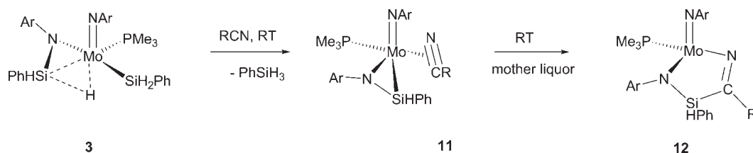
Scheme 6. Reactions of 3 with Nitriles
