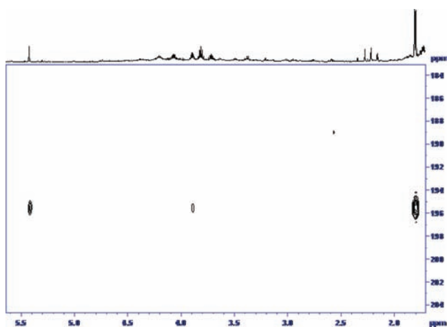
Figure 5. ^1\text{H} – ^{13}\text{C} HMBC NMR spectrum of 12c taken directly from the reaction mixture. Signals at 5.4, 3.9, and 1.8 ppm correspond to the SiH, CH, and \text{CH}_3 protons, respectively.
