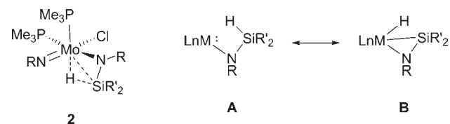
Chart 1. Valence Bond Description of Bonding in Agostic Complexes 2
