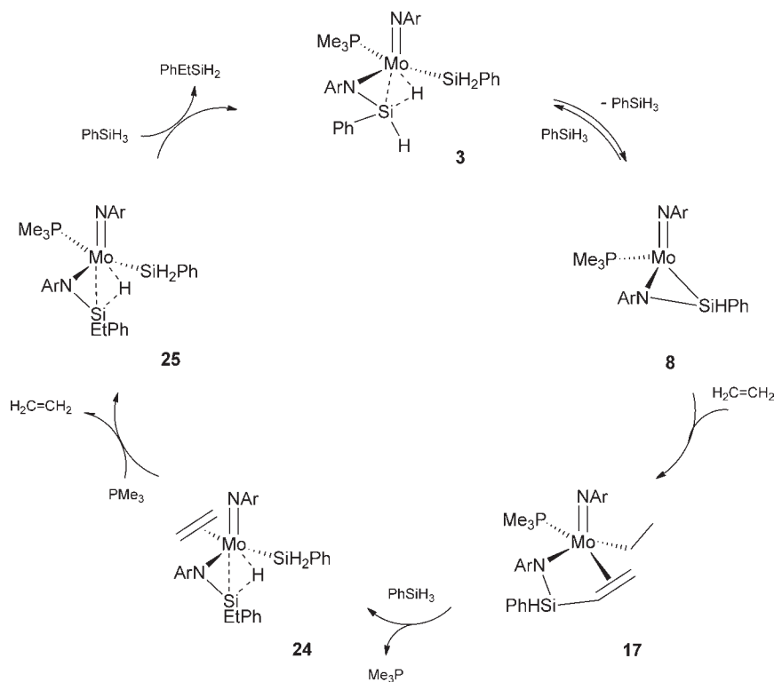
Scheme 17. Possible Catalytic Cycle for the Hydrosilylation of Ethylene by PhSiH 3 Mediated by 3
