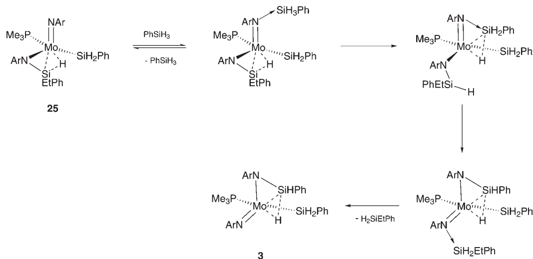
Scheme 16. Suggested Mechanism for the Reaction of 25 with Excess \text{PhSiH}_3
