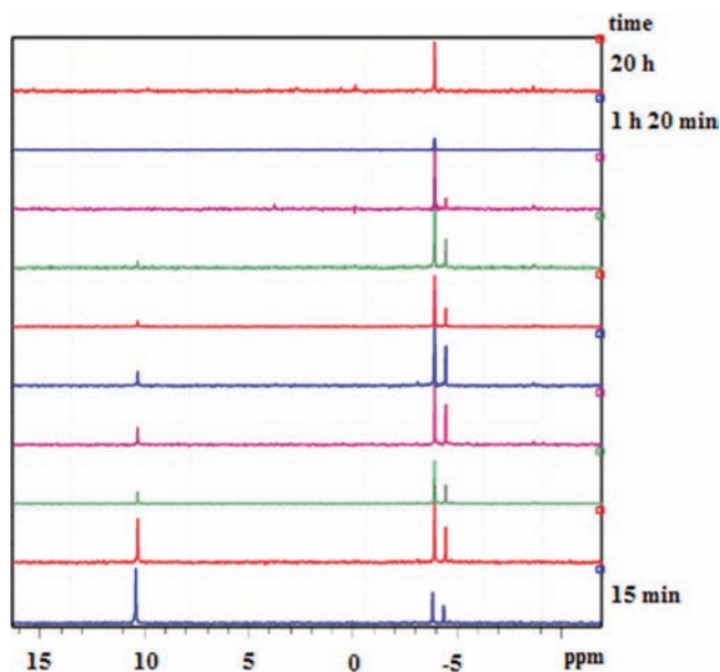
Figure 4. 31 P{ 1 H}-NMR spectra of the reaction mixture of 3 and t PrCN (the signals at 10.5, –3.8, and –4.4 ppm correspond to 3 , 12d , and 11d , respectively).
