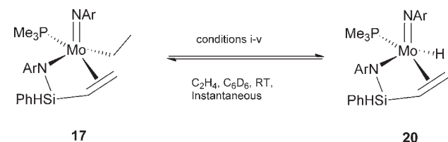
Scheme 13. Thermal Stability of 17 and Its Reactions with Hydrosilanes and \text{H}_2 a
